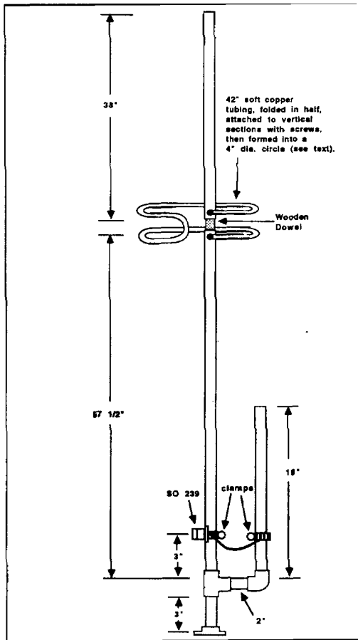
Figure 1. Dimensions for the Super J-Pole.
